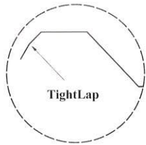
PBR Panel w/ TightLap Used for roof and wall applications. Minimum Slope is 1/2:12.
